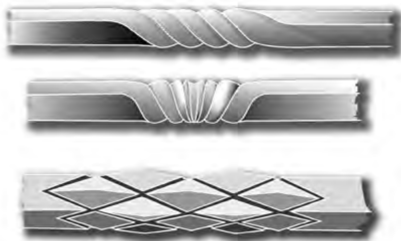
Top, simple cold twist. Middle, progressive reverse twist, made hot. Bottom, pineapple twist, made by twisting, hammering and untwisting, all at an incandescent heat.
