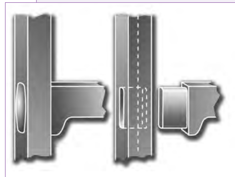
Mortises and tenons resemble their wooden counterparts. In this example, the tenon is made longer than the mortise, and pinned or headed like a rivet to draw the joint tight and secure it. Sometimes captive wedges are used.
